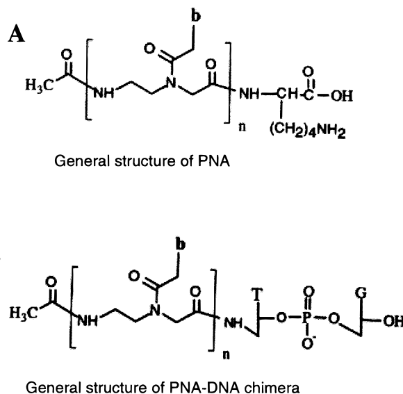
FIGURE 1: Structure for (PNA) 21 and (PNA) 19 -TpG-OH chimera. The sequences of (PNA) 21 and (PNA) 19 -TpG-OH chimera are shown in Chart 1. In the figure, b represents A, T, G, or C purine and pyrimidine bases linked with polyamide backbone and n represents the number of these bases in the molecule. (PNA) 21 has a single Lys amino acid at the end of (pseudo 3' terminus) the sequence while the (PNA) 19 -TpG-OH chimeric molecule is comprised of 19 bases in the form of PNA followed by a normal dinucleotide TpG with G having a free 3'OH terminus.
